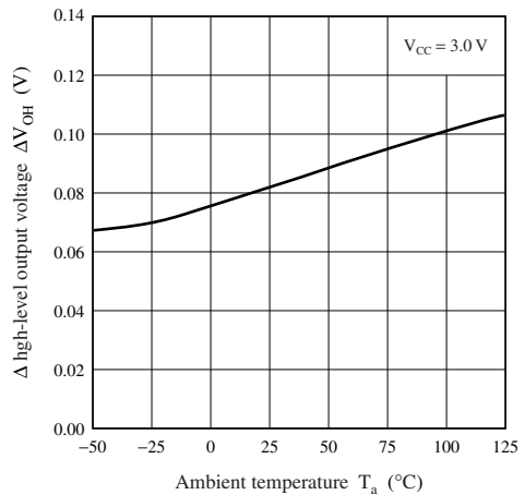
\Delta high-level output voltage — Ambient temperature
